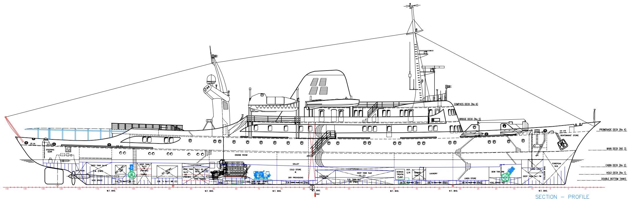
SECTION - PROFILE
